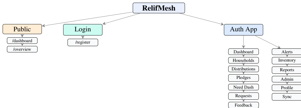
Figure 17: RelifMesh Information Architecture
